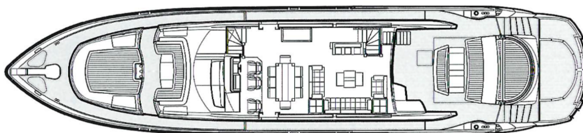
Main deck
