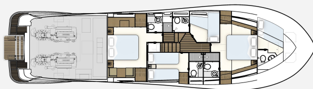
Lower Deck - 3 cabins
